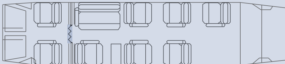
KING AIR B200 CABIN CONFIGURATION
